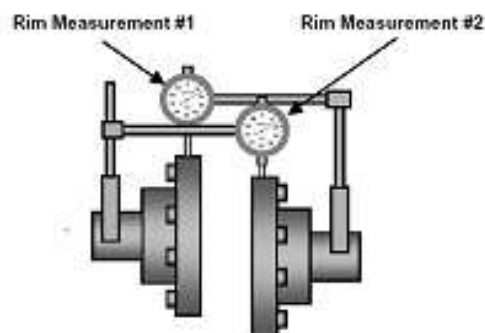
Gambar 5. Metode reverse indicator
