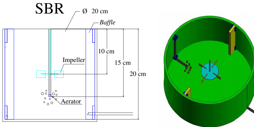
Gambar 1 Sketsa Reaktor SBR
