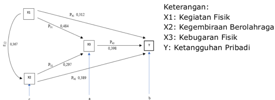
Gambar 1. Model pasca uji korelasi bivariat
