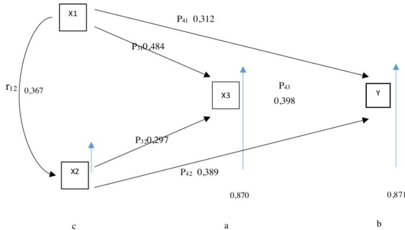
Gambar 4. Model hipotesis ketiga
