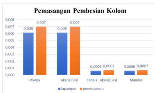
Figure 4. 1 Comparison Chart of Column Ironing Installation Coefficient Value
