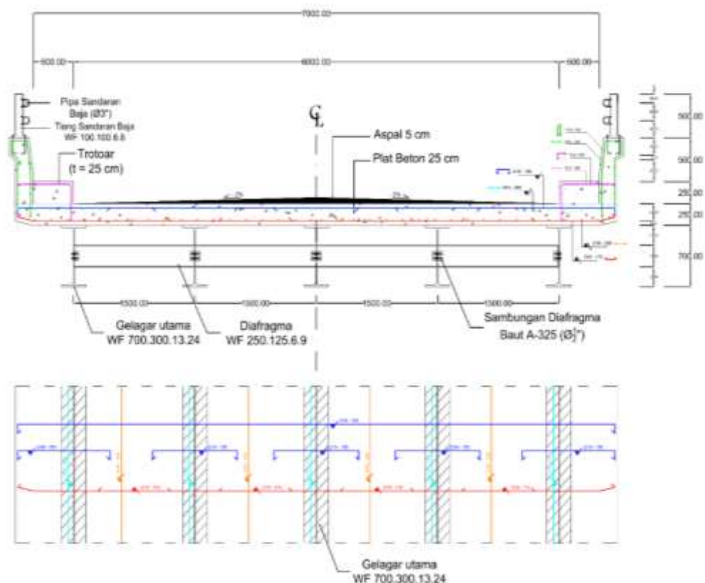
Figure 4.1 Details of Reinforcement of Vehicle Floor Slabs, Pavement and Parapets
