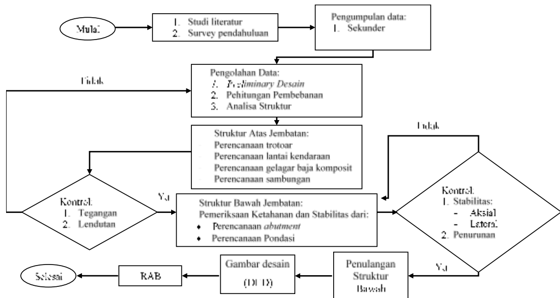
Figure 3.1 Design Flowchart
