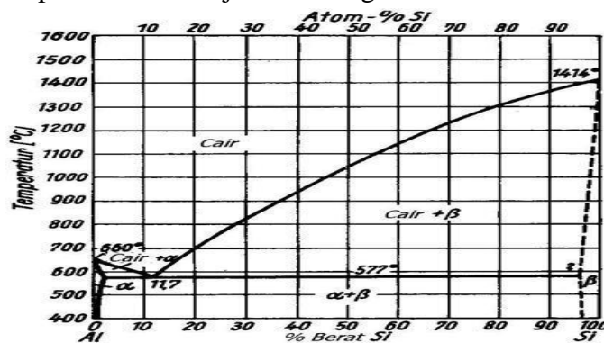
Gambar 6. Diagram Fasa Al-Si
